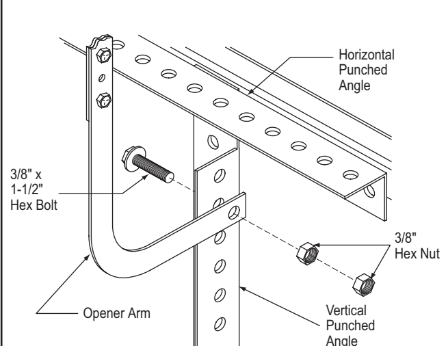
Top View (assembled)
