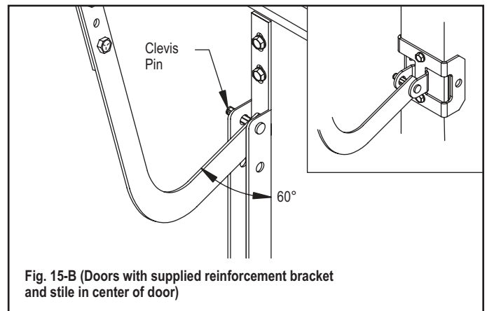
Opener Arm Attachment to Vertical Angle
